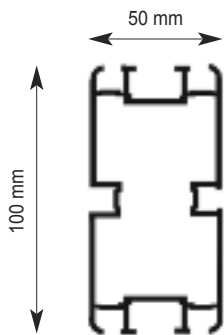
Gamba intermedia
